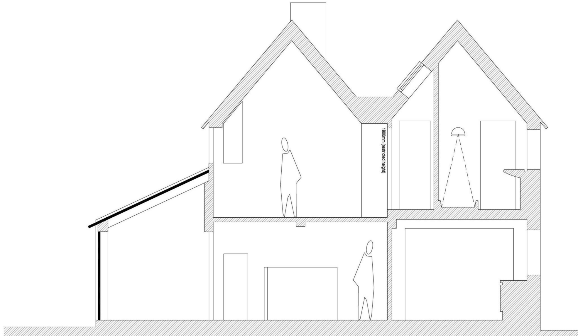
Proposed Section (main dwelling)
