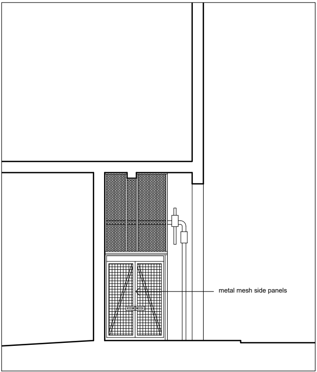
SIDE ELEVATION FROM EAST STREET
