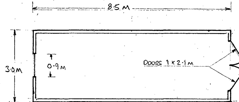
FLOOR PLAN
