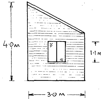
LH SIDE ELEVATION
