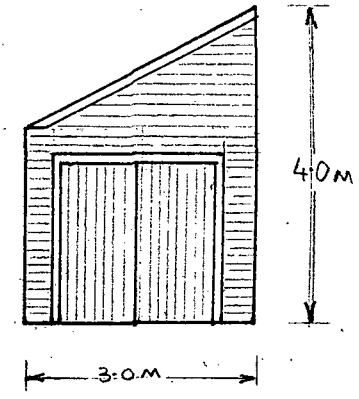
RH SIDE ELEVATION
