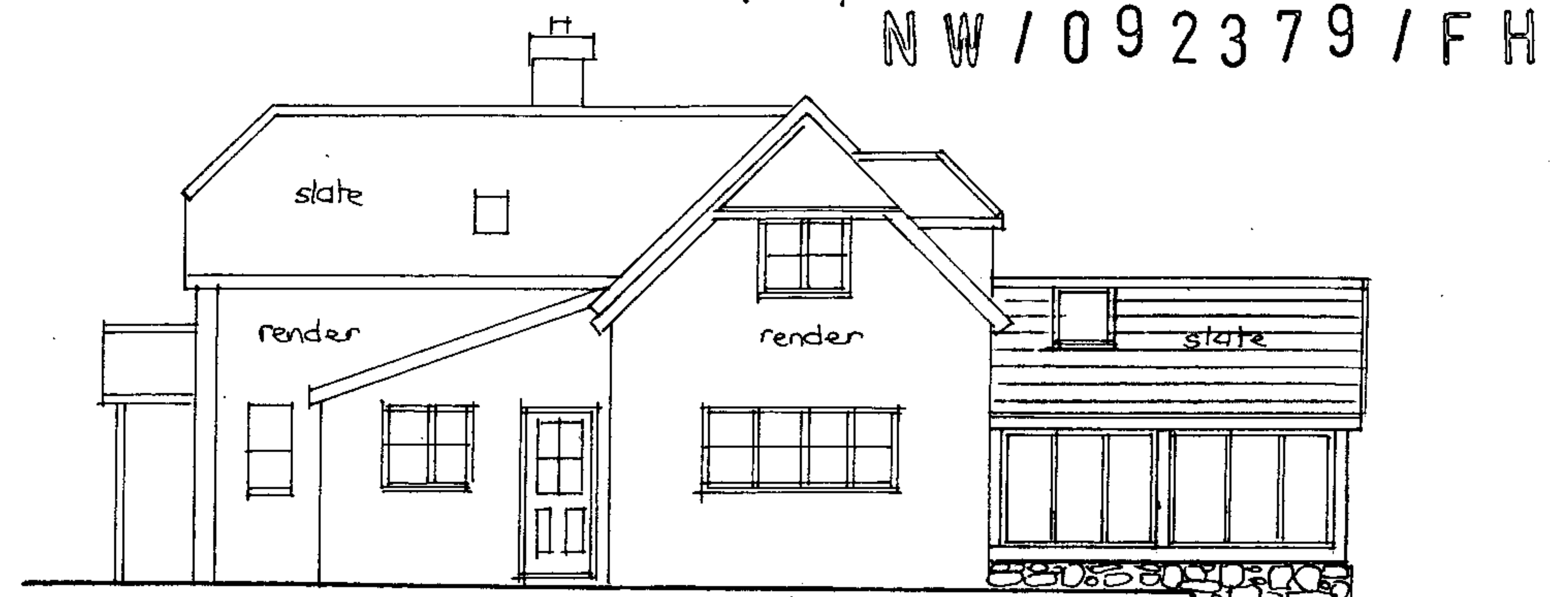
west elevation
