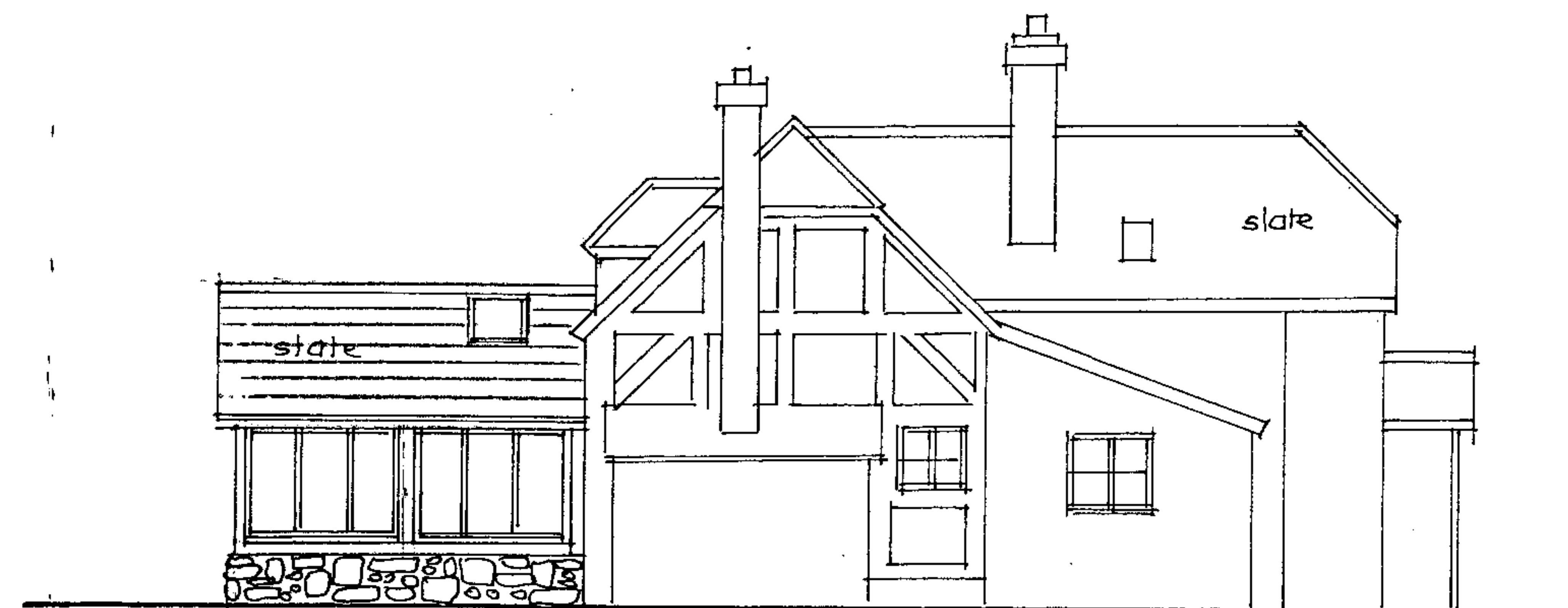
east elevation
