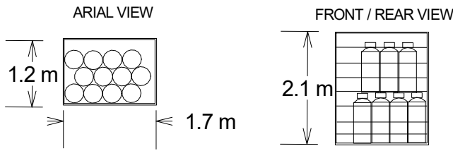
PROPANE AND BUTANE CYLINDER STORAGE IN A STILLAGE (CAGE)
