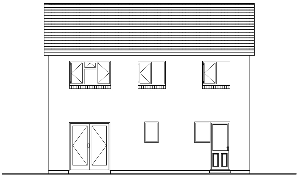
Rear Elevation
