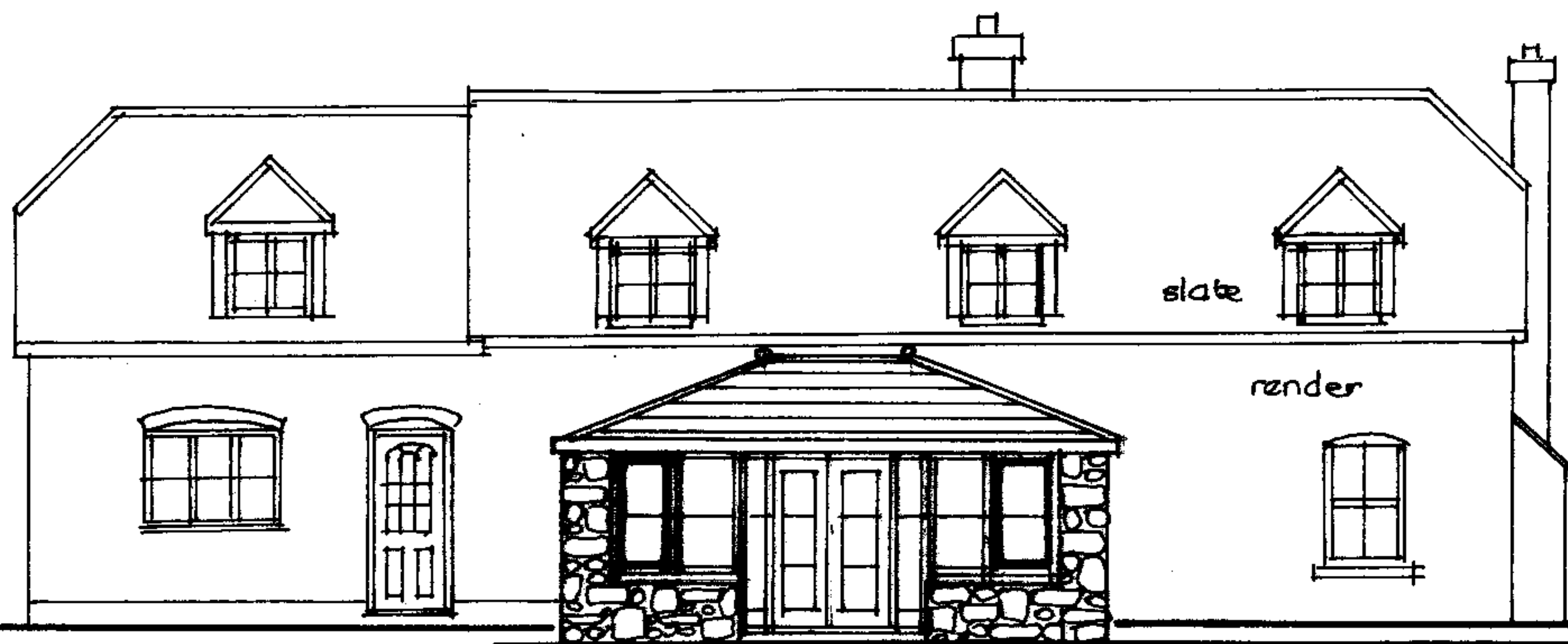
south elevation
