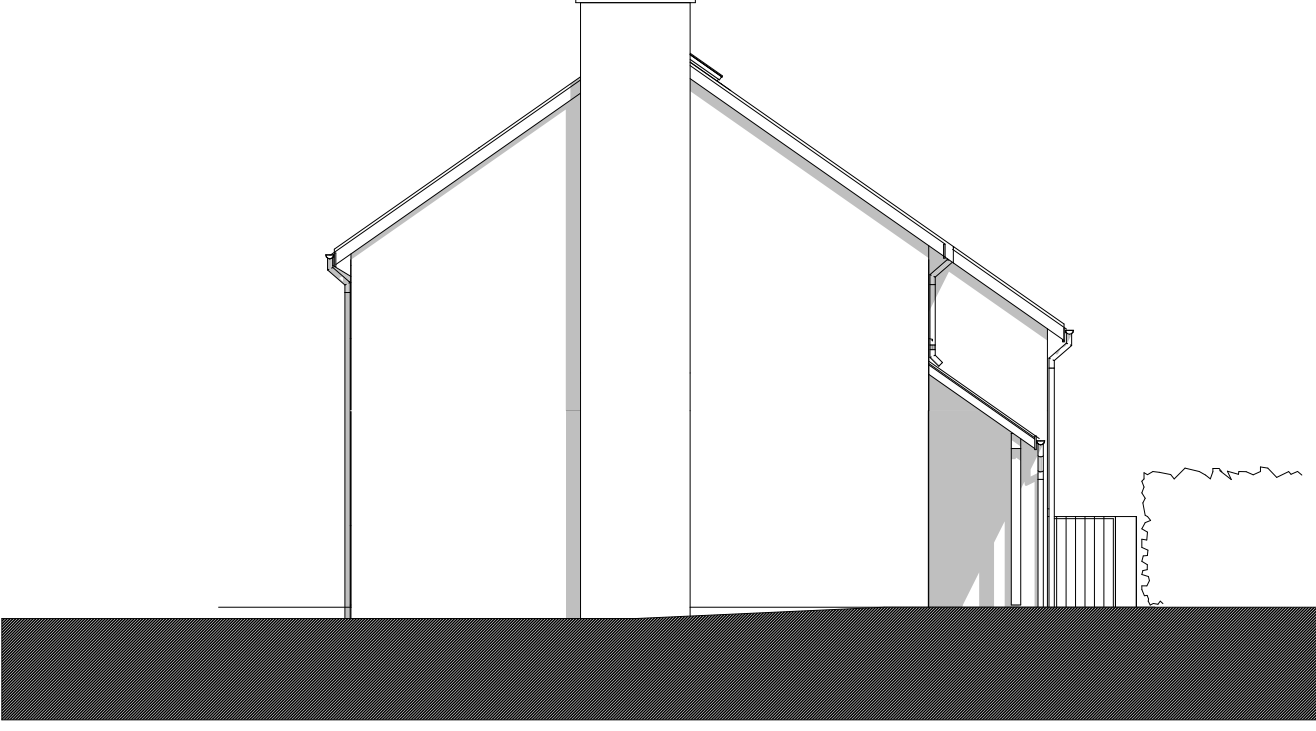
4. WEST ELEVATION
