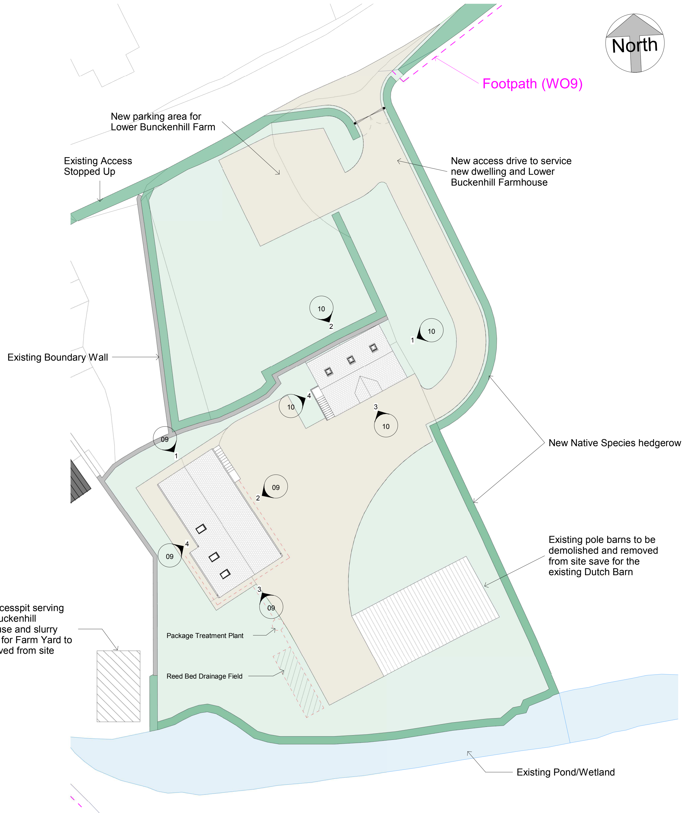
B2 Proposed Site Plan 1 : 200
