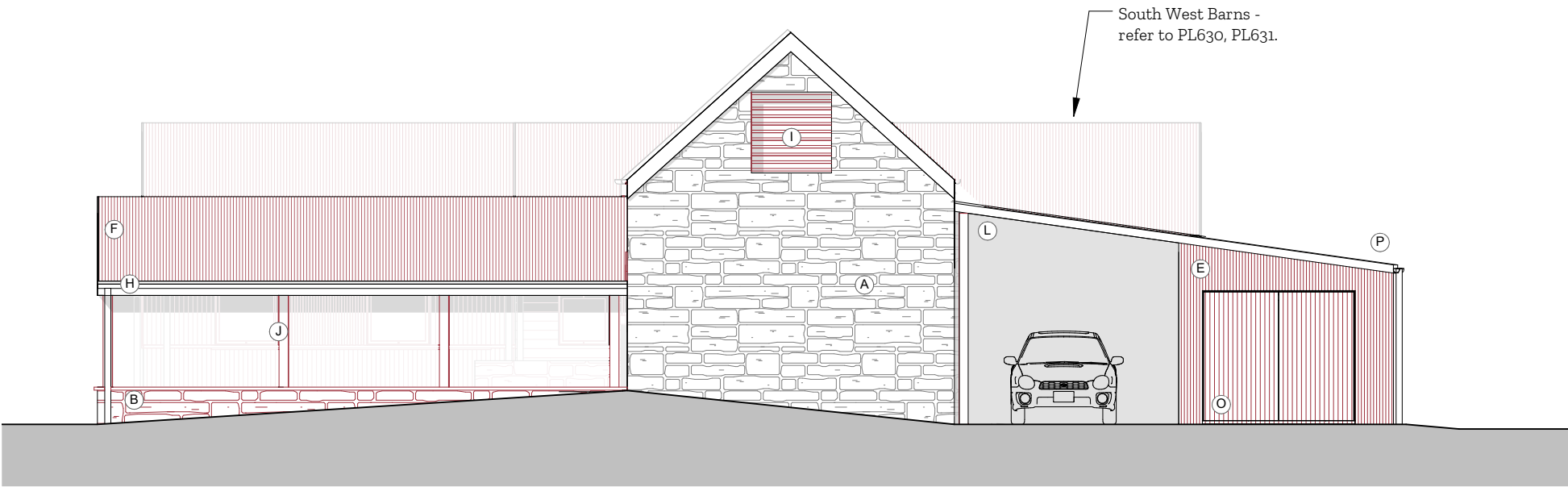
① North Elevation - Linhay 1:100
