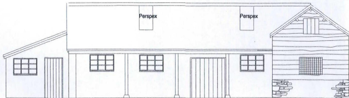
EAST ELEVATION
